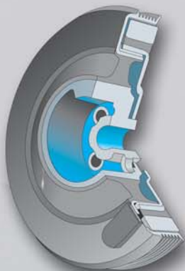
Torsional Vibration Damper Isolator (TVDi)
